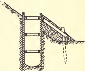
FIG. 32.—SHEATHING ON STEEP SLOPES.
